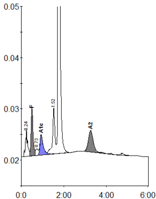
Peak table - ID: A1355488
