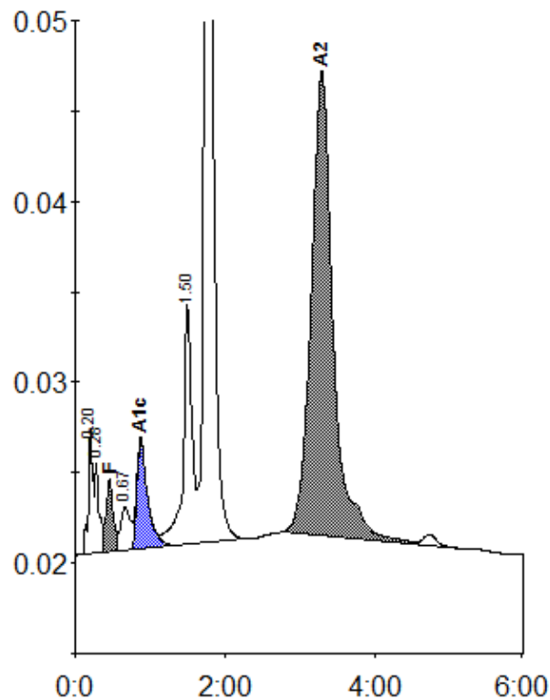
Peak table - ID: A1482978
