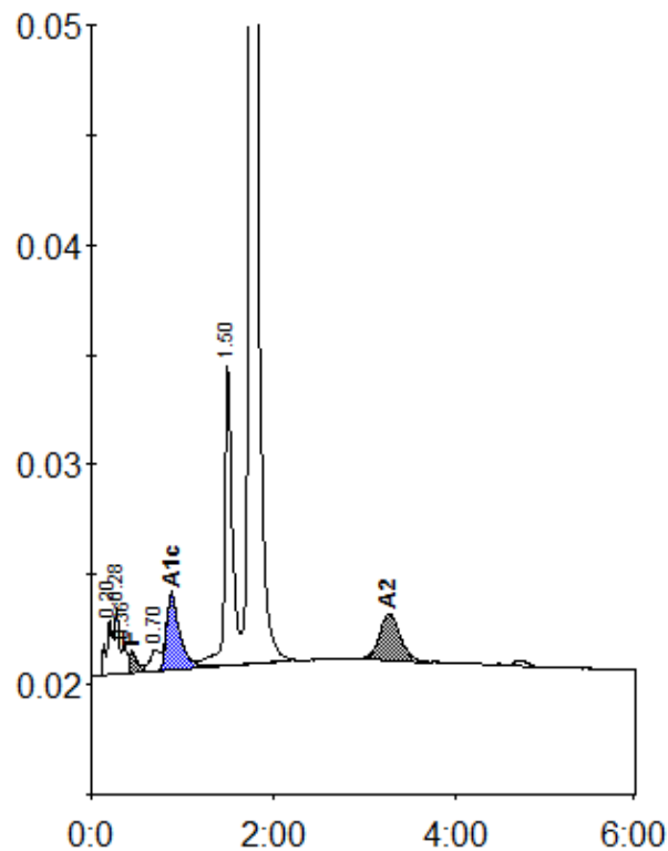
Peak table - ID: A1511087
