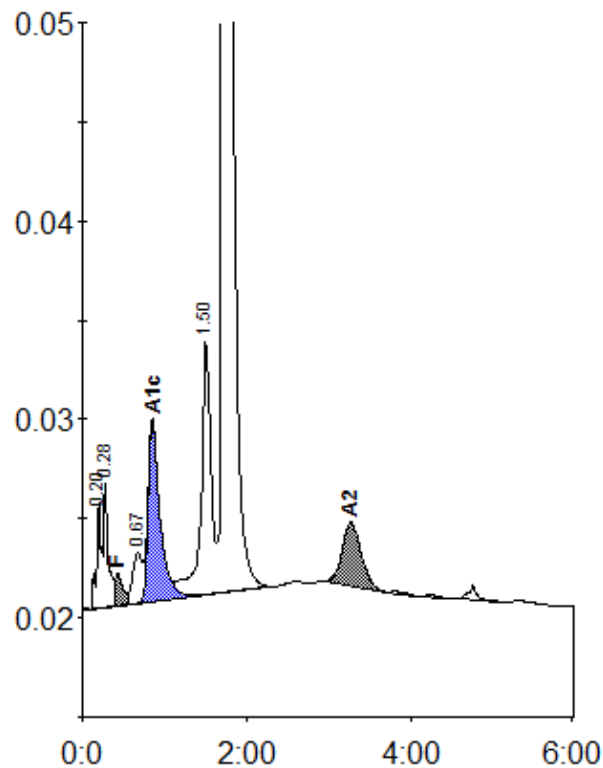
Peak table - ID: A1993114
