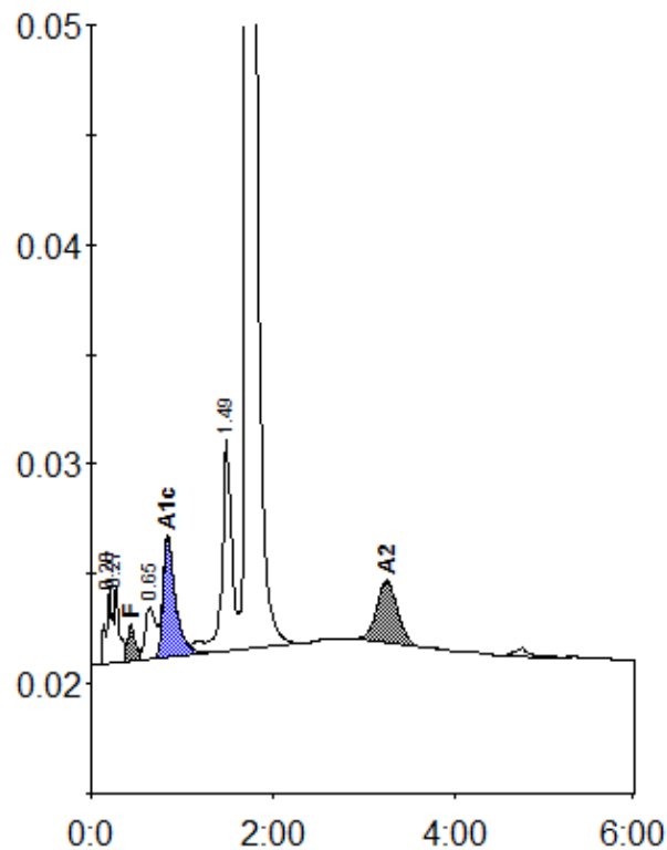
Peak table - ID: A1644228
