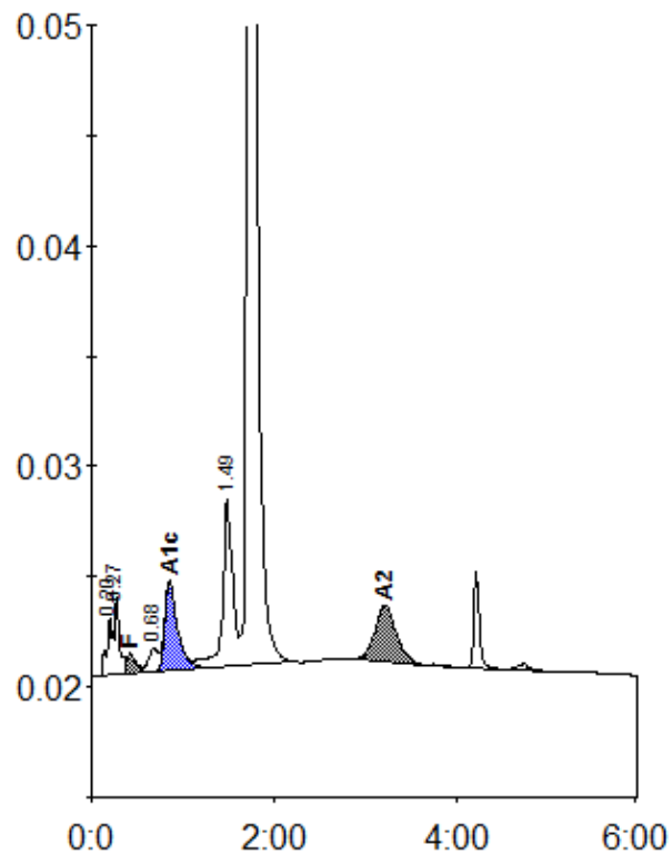
Peak table - ID: A1630813
