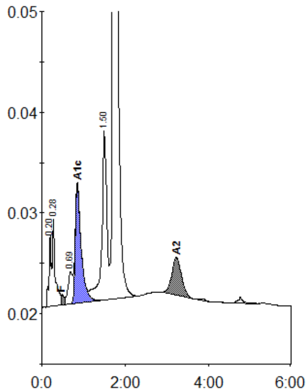
Peak table - ID: A2092236
