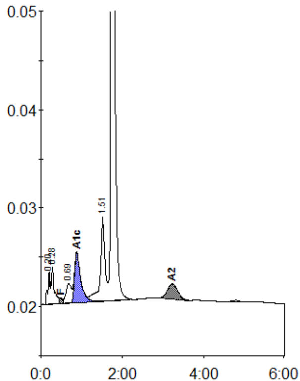
Peak table - ID: A1007323
