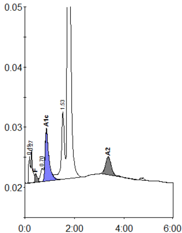
Peak table - ID: B2664387
