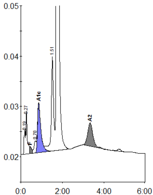
Peak table - ID: A1913826
