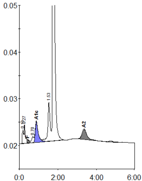
Peak table - ID: A2203224
