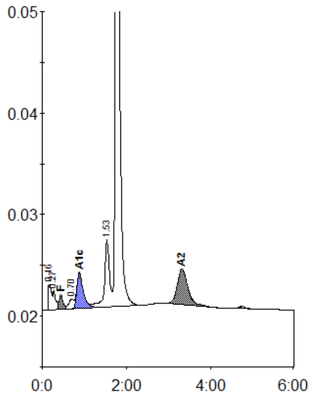
Peak table - ID: A1623195
