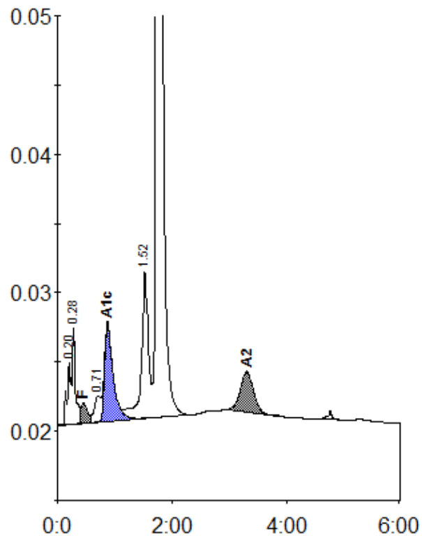
Peak table - ID: B2603611
