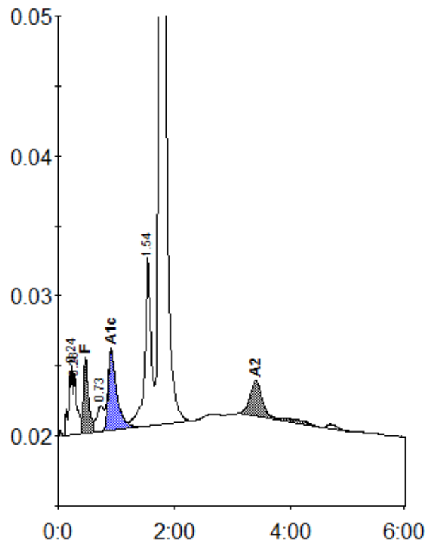
Peak table - ID: B2952096
