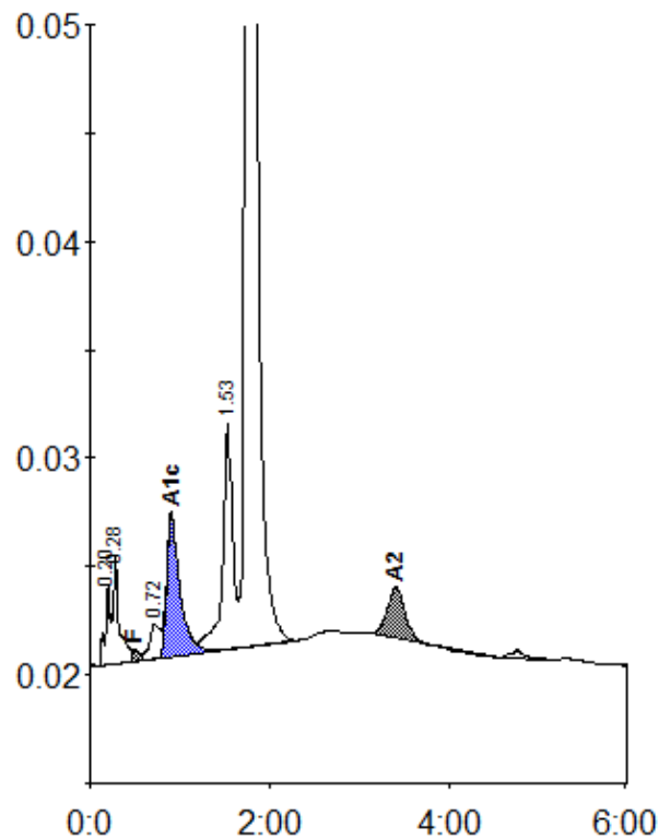
Peak table - ID: B2797434
