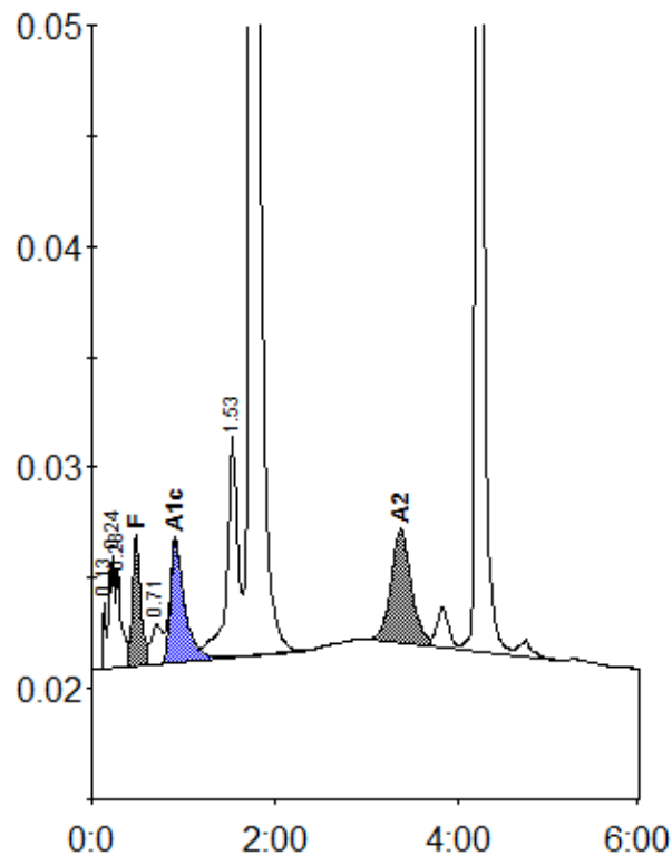
Peak table - ID: A1547117
