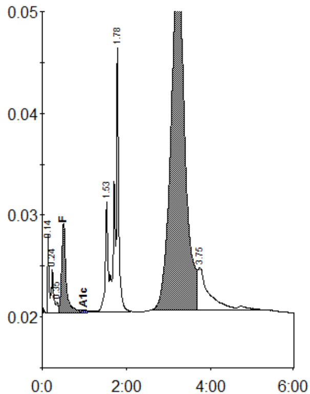
Peak table - ID: B2558520
