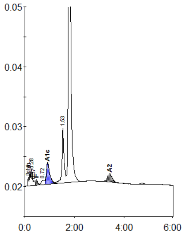
Peak table - ID: B2838200
