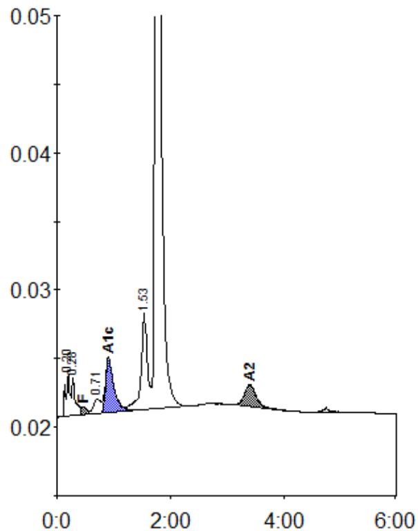
Peak table - ID: B2837884
