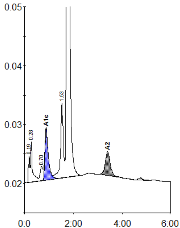
Peak table - ID: B2404762
